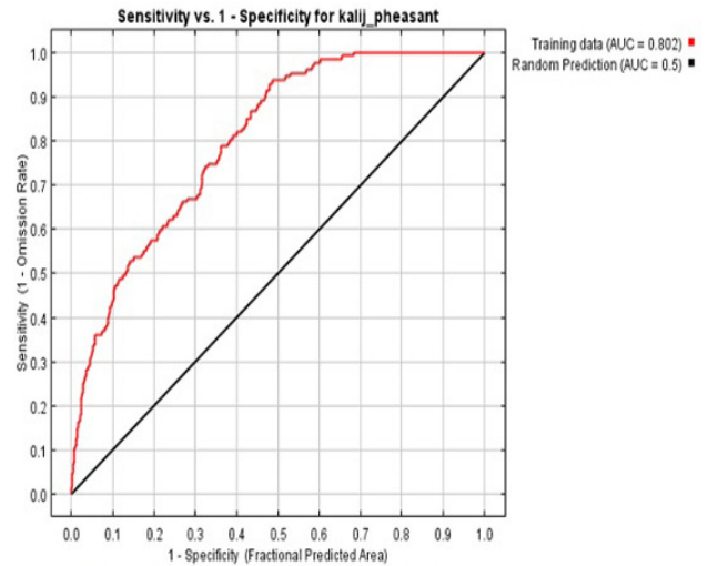
Fig. 3. AUC sensitivity and specificity for kalij pheasant.
