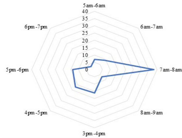
Fig. 2. Activity pattern of kalij pheasant in study area.
