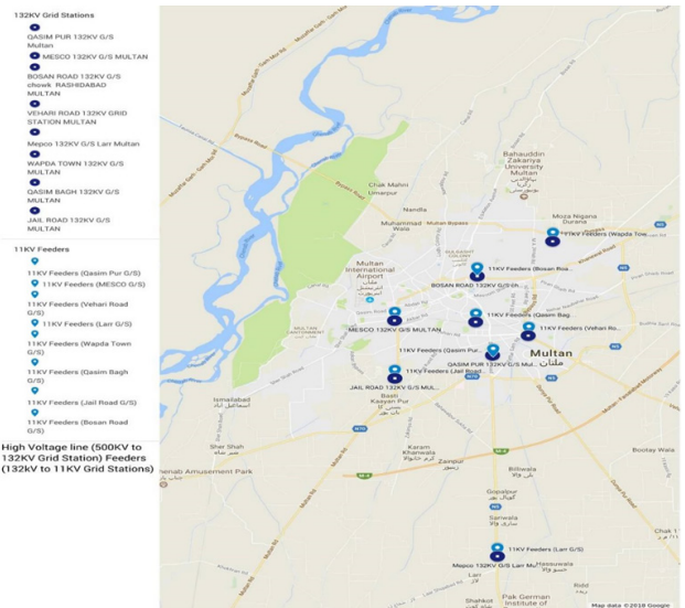
Fig. 6. Locations 132kV high voltage grids and 11kV outgoing feeders in Multan.
