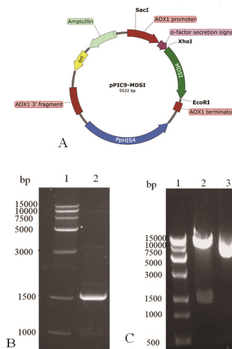
Fig. 1. Construction of the expression vector pPIC9- \alpha -M, A) schematic diagram of the expression vector pPIC9- \alpha -M; B) PCR amplification of mds I gene from pAO815 \alpha -M, molecular marker (lane 1), mds I gene (lane 2); C) identification of pPIC9- \alpha -M by enzyme digestion, molecular marker (lane 1), pPIC9- \alpha -M digested by Eco R I and Xho I (lane 2) and circle plasmid pPIC9- \alpha -M as control (lane 3).
