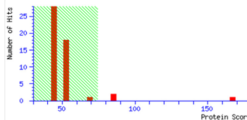
Fig. 4. PMF analysis of the expressive product.
