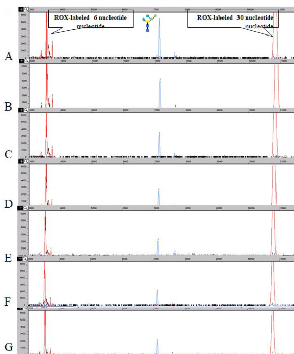
Fig. 8. The effect of metallic ions on the activity of MDS I, \text{Cu}^{2+} (A), \text{Co}^{2+} (B), \text{Zn}^{2+} (C), \text{Mn}^{2+} (D), control (E), \text{Mg}^{2+} (F) and \text{Ca}^{2+} (G).
