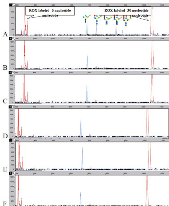
Fig. 7. The effect of temperature on the activity of MDS I, control (A), 16 °C (B), 25 °C (C), 37 °C (D), 42 °C (E) and 60 °C (F).
