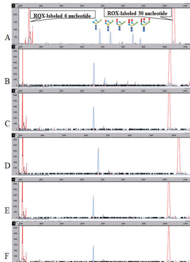
Fig. 6. The effect of pH on the activity of MDS I, control (A), pH 3.0 (B), pH 5.0 (C), pH 7.0 (D), pH 9.0 (E) and pH 11.0 (F).
