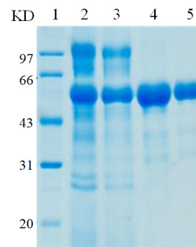
Fig. 3. SDS-PAGE analysis of the purified MDS I, molecular marker (lane 1), 10 µL MDS I from raw liquid (lane 2) and each elution after purification from ammonium sulphate precipitation (lane 3), Phenyl-HP (lane 4), Sephadex G25 (lane 5) was subjected to the 12% SDS-PAGE and stained by Coomassie blue.
