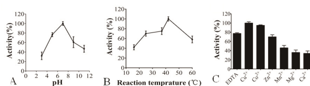
Fig. 9. The influence of pH (A), temperature (B), cation (C) on the reaction of RNase B N-glycans catalyzed by MDS I.
