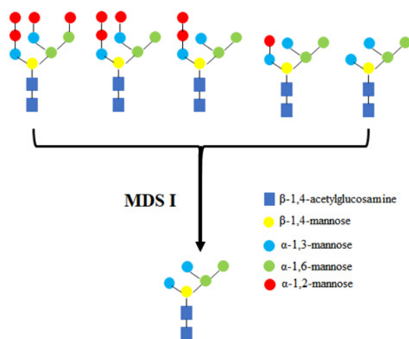
Fig. 5. Five glycoforms of RNase B and MDS I catalyze reaction.
