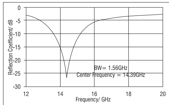
Fig 2: Return loss of Reference patch antenna
