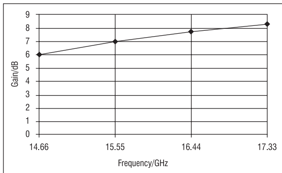
Fig 11: Gain of the antenna
