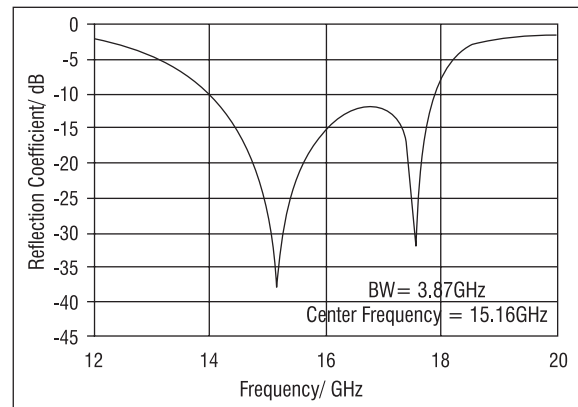
Fig 4: Return Loss of the proposed antenna
