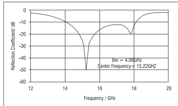
Fig 8: Return loss of optimized antenna
