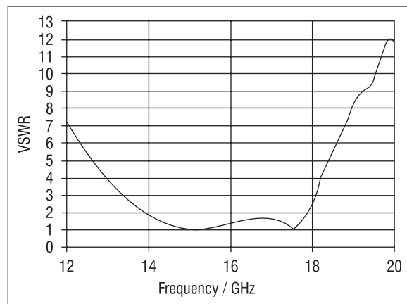
Fig 5: Voltage Standing Wave Ratio
