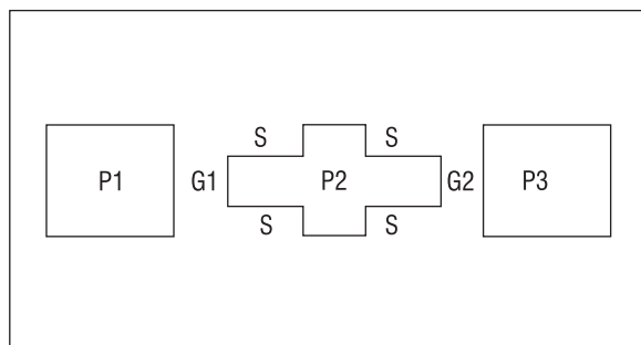
Fig 3: Front View of the Proposed Antenna
