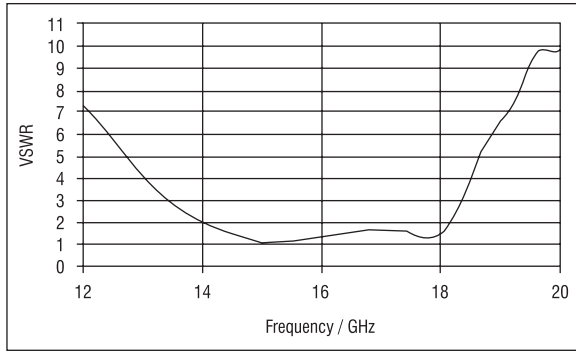
Fig 9: VSWR of the antenna
